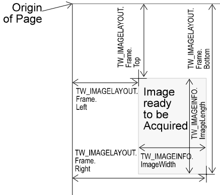
Figure 4-1. TW_FRAME Structure
