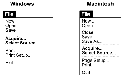
Figure 3-1. User Interface for Selecting a Source and Acquiring Options
