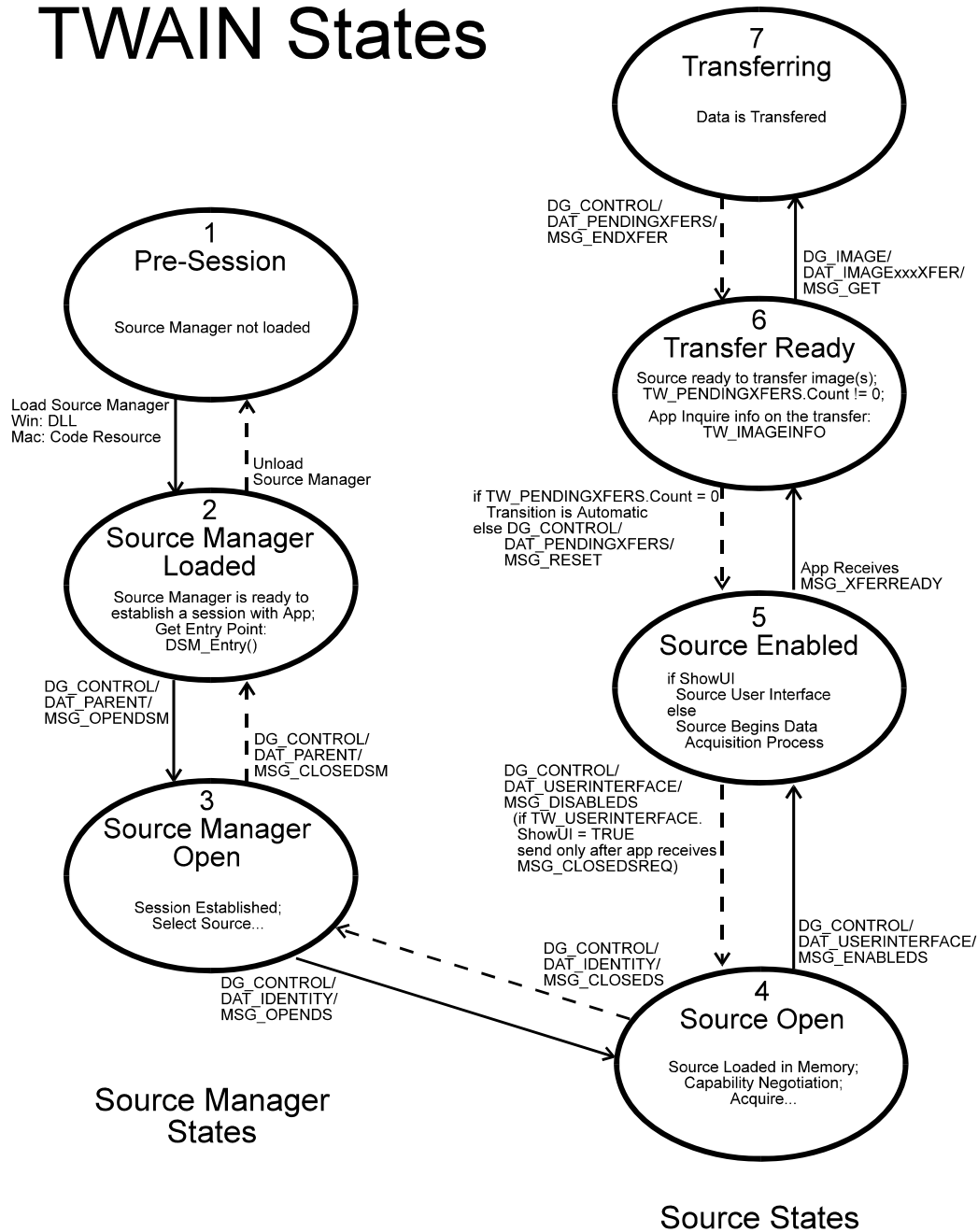
Figure 3-2 TWAIN States
