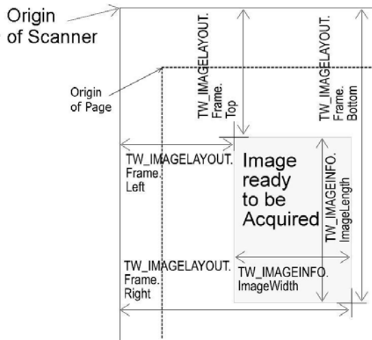
Figure 4-1. TW_FRAME Structure
